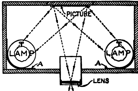
FIG. 341. — Plan of Reflectoscope.
